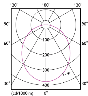
GU10 7.5-80W 650lm 120D 3000K GU10 D
